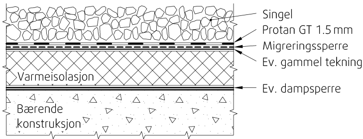
Fig. 1 Ballastert, isolert rettventd tak, nyteking/omteking
